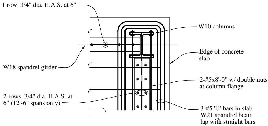
Figure 9.2-3 Typical corner PRCC
