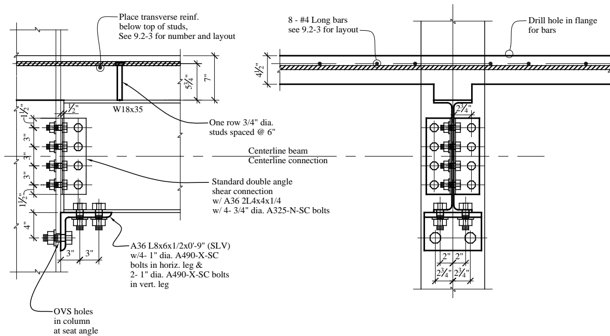
Figure 9.2-1 Typical interior W18x35 PRCC
