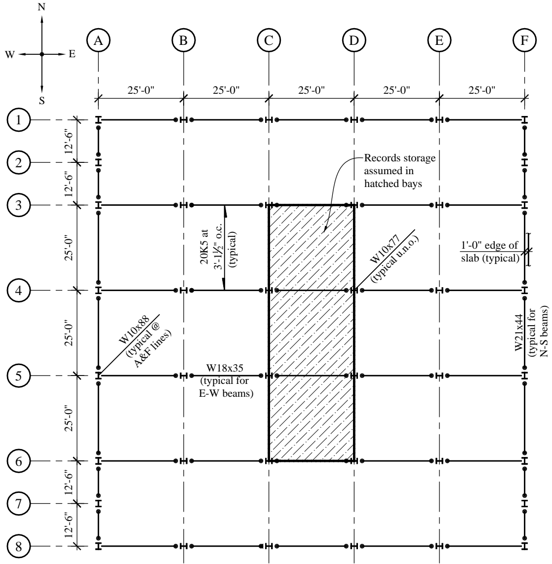
Figure 9.1-1 Typical floor and roof plan
