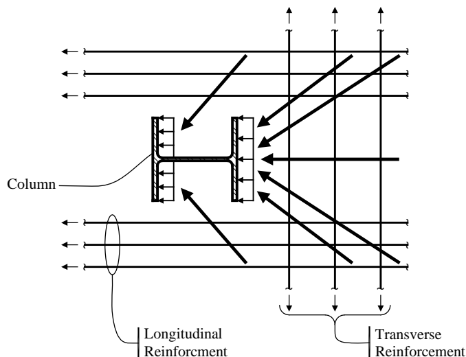
Figure 9.2-7 Force transfer mechanism from slab to column
