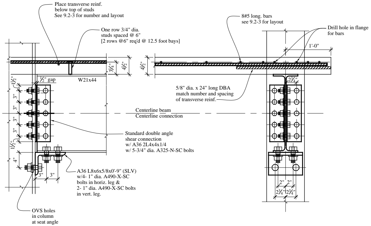
Figure 9.2-2 Typical spandrel W21x44 PRCC
